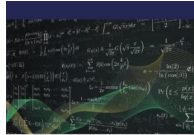
Multi layer model for correlated energy prices
