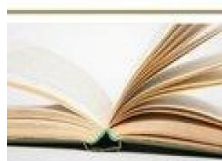
Superconductivity and Magnetism in Iron Arsenides and Cuprates
