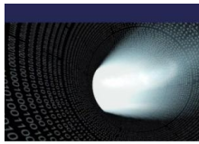
Numerical Methods for Solving Semi-infinite Optimization Problems
